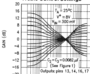
Tone Control Response with Reciprocal Bass and Treble Control Settings
