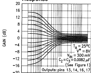
Bass Tone Control Response
