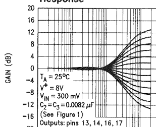
Treble Tone Control Response
