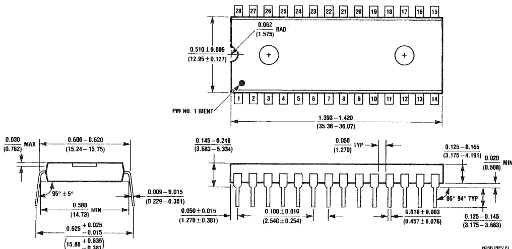
Molded Dual-In-Line Package (N) Order Number LMC1992CCN NS Package Number N28B
