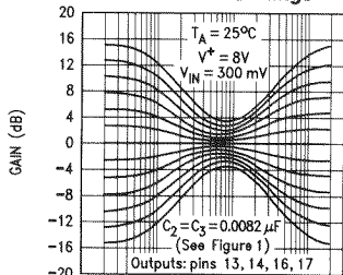
Tone Control Response with Equal Bass and Treble Control Settings
