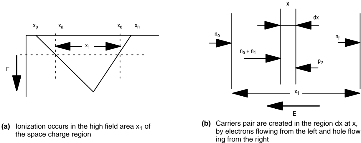
Figure 2. Ionization Process Location for a Non Punch Trough Structure
